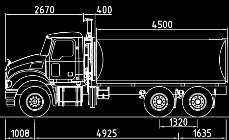
METRO-LINER 6X4 WATER TANKER
