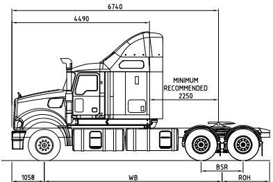
60" Sleeper (1,524mm)
